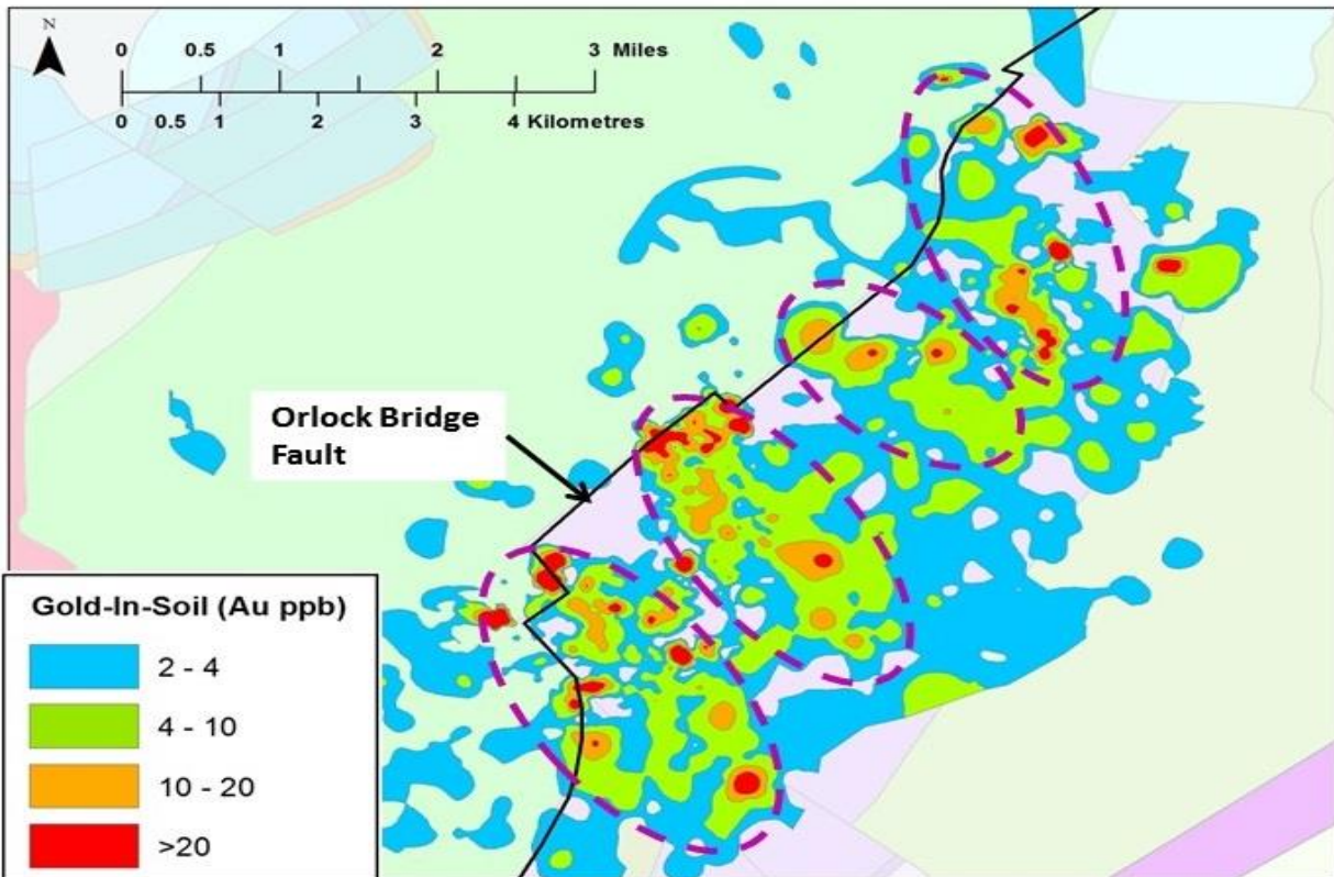
Exhibit 2: Slieve Glah geology and Gold Target Anomalies
